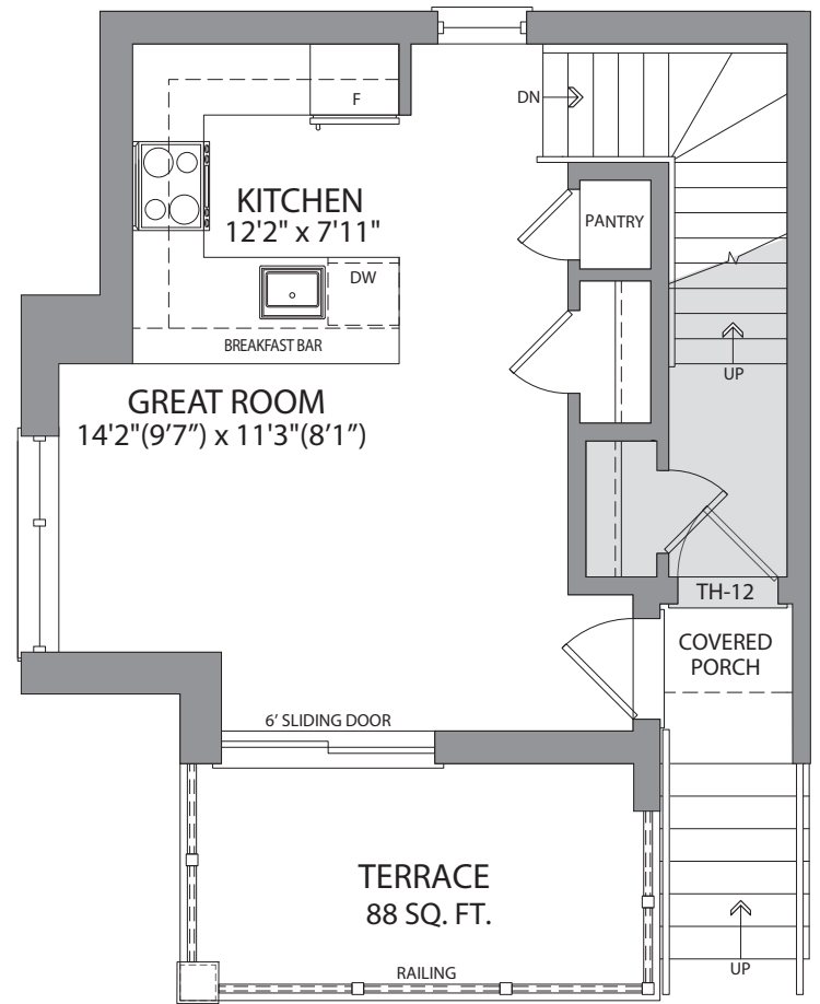
GROUND FLOOR ELEVATION A & B
