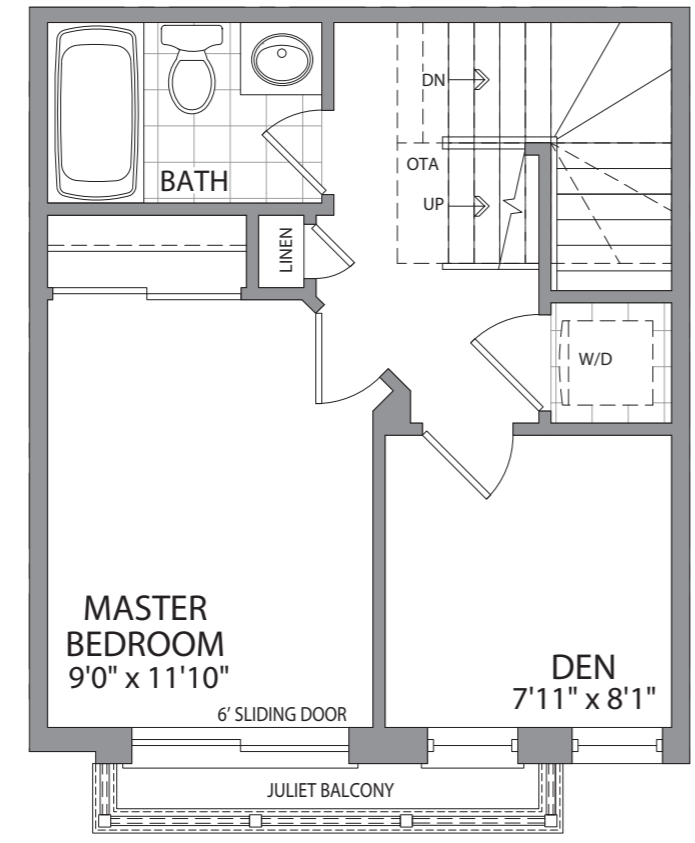
THIRD FLOOR ELEVATION A
