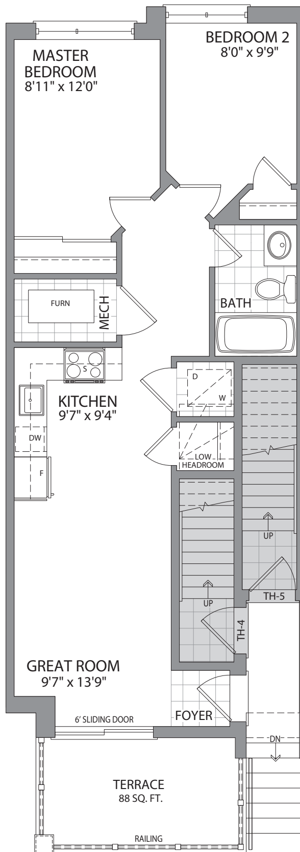
GROUND FLOOR ELEVATION B
